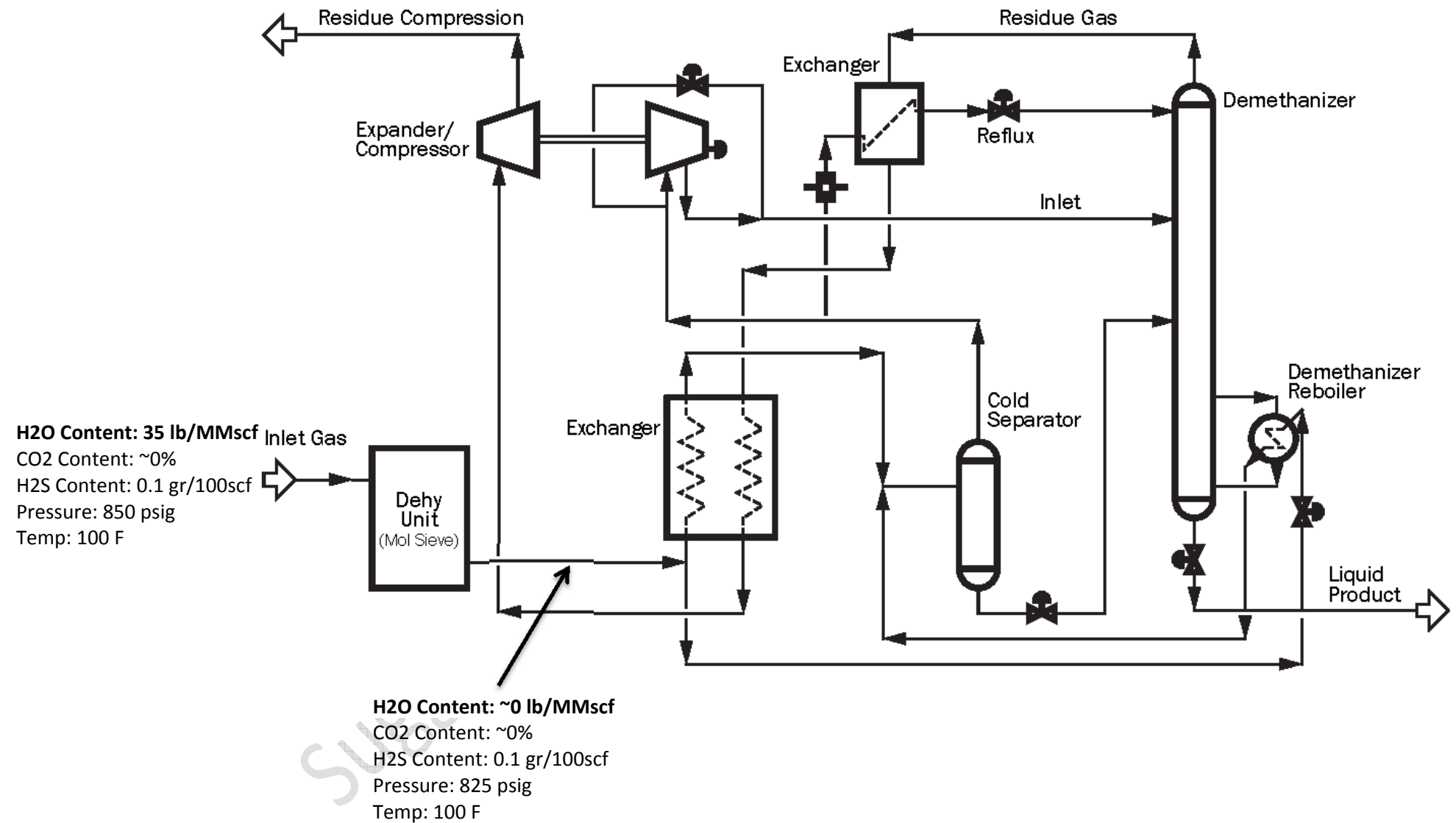
Figure 1: PFD
